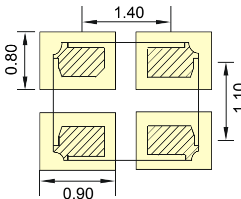
推荐的焊盘布局 Recommended Solder Pad Layout
